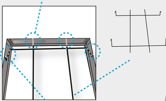
Wire support grid into filter frame
